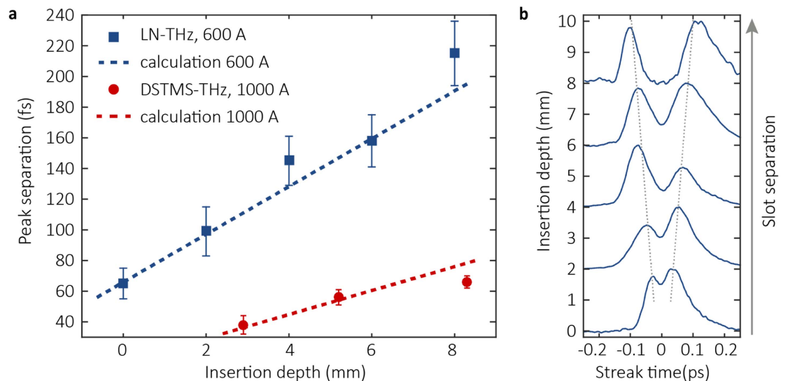
Figure 5. Control over the x-ray pulse structure. The double-slotted spoiler was scanned for two different compression factors in the magnetic chicane (600 and 1000 A). LN-THz is used to measure x-ray pulses generated with the lower compression factor, and DSTMS-THz (with higher temporal resolution) to measure pulses with the higher compression factor. In panel (a), as expected, the delay between the x-ray pulse pairs varies linearly with the lateral distance between the slots in the emittance-spoiling foil. In practice, the separation is controlled with the insertion depth of the foil in the centre of the chicane. For these simple x-ray pulse shapes, the calculated delay based on simulation of the linear accelerator is in excellent agreement with the observed delay. Panel (b) shows characteristic single-shot measurements obtained using the lower compression setting at five different insertion depths. The dotted lines indicate the expected linear dependence.
