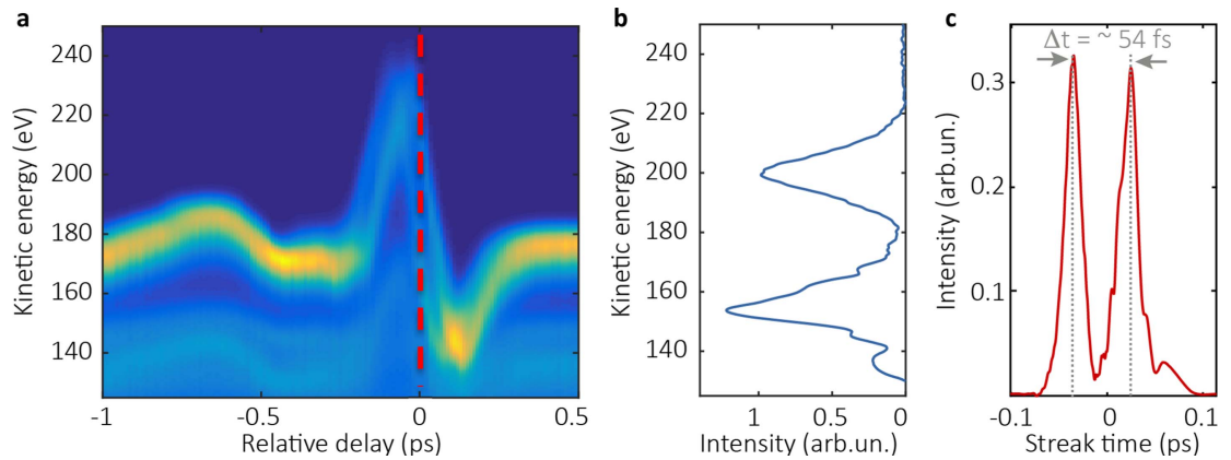
Figure 4. High resolution temporal characterization with DSTMS-THz pulses. The spectrogram shown in panel (a) contains single-shot spectra averaged according to the set relative delay between the x-ray FEL and THz pulses, plus a correction provided by the spectral encoding time-tool (see Methods). The x-ray photon energy was 1.04 keV. Due to the x-ray pulse structure imprinted by the double-slotted spoiler, the streaked photoelectron spectrum splits into two distinct peaks near time-zero. A characteristic single-shot spectrum at zero delay is shown in panel (b). The corresponding x-ray temporal pulse profile is retrieved and shown in panel (c). In this case, the two x-ray pulses are separated by \sim 54 fs.
